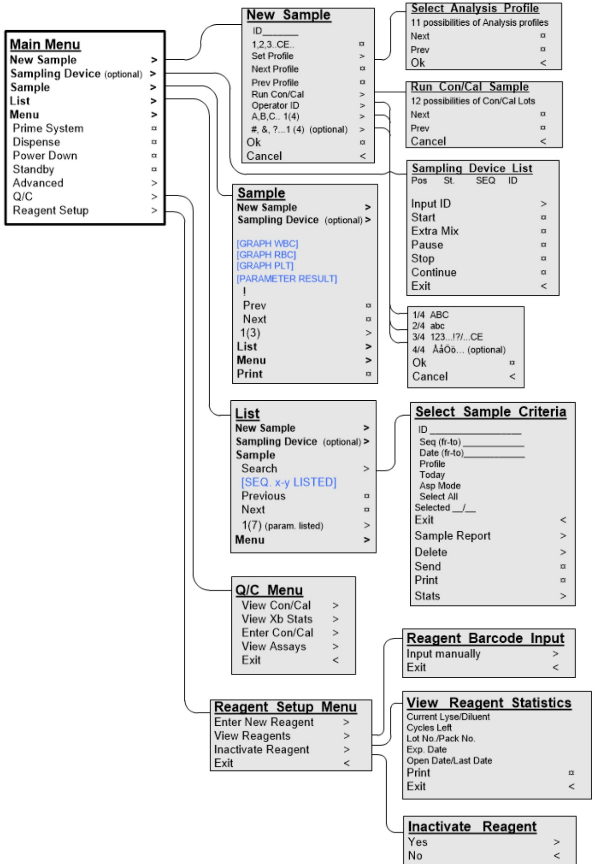
Flowchart 3.1 Main Menu Structure
